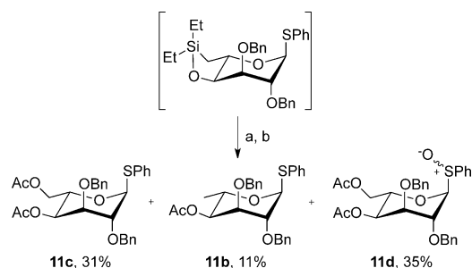
Scheme 2. Fleming–Tamao oxidation to obtain the L-altroside. Reaction conditions: a) UHP (30 equiv), KF (3 equiv), \text{KHCO}_3 (5 equiv), DMF, 50 °C, 3 h; b) \text{Ac}_2\text{O} , DMAP, \text{CH}_2\text{Cl}_2 , \text{Et}_3\text{N} . Yields over four steps. UHP = urea/hydrogen peroxide complex.
