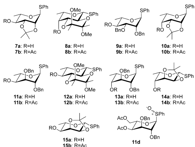
Figure 1. 6-Deoxy L-thio-glycosides used in the synthesis of the L-hexoses, the protodesilylation by-products and the sulfoxide side product 11d.
