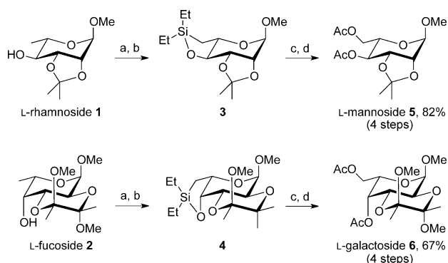
Scheme 1. Synthesis of methyl L-pyranosides from their corresponding 6-deoxy L-hexoses. [29] Reaction conditions: a) \text{Et}_2\text{SiH}_2 , [\text{Ir}(\text{cod})\text{OMe}]_2 (0.5 mol %), THF, RT, 13–16 h; b) [\text{Ir}(\text{cod})\text{OMe}]_2 (2 mol %), \text{Me}_4\text{Phen} , norbornene, THF, 24–28 h, 120 °C; c) 30% \text{H}_2\text{O}_2 , \text{KHCO}_3 , THF/MeOH (1:1), 50 °C, 6 h; d) \text{Ac}_2\text{O} , DMAP, \text{CH}_2\text{Cl}_2/\text{Et}_3\text{N} , RT, 1 h. \text{Me}_4\text{Phen} = 3,4,7,8-tetramethyl-1,10-phenanthroline.
